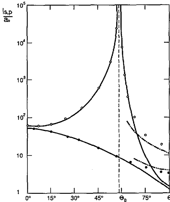
Figure 1. The dependence of the localization length on the angle of light incidence at \lambda = 5a_0 , n^2 = \varepsilon_2/\varepsilon_1 = 2.42 . Open circles are the results of Monte Carlo simulations for p-polarized light, and the full circles are for s-polarized light according to [22]. Full curves are calculated from equation (42). The chain curves display the results of equation (43).
